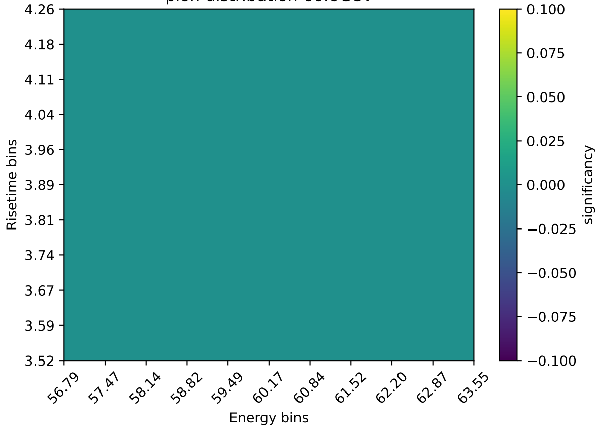
pion distribution 60.0GeV
